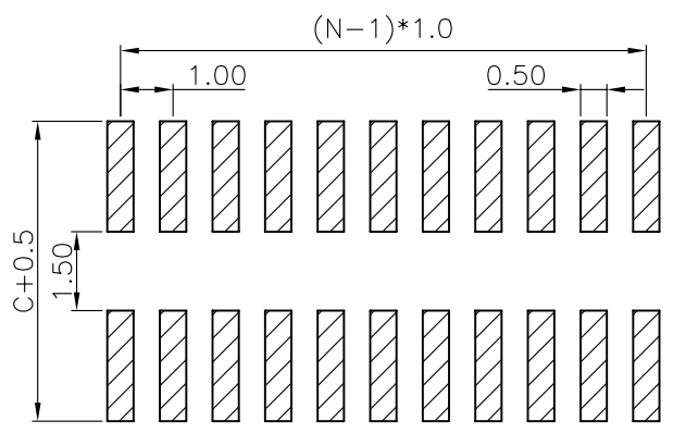
RECOMMEND PCB LAYOUT(TOLERANCE=±0.05)
